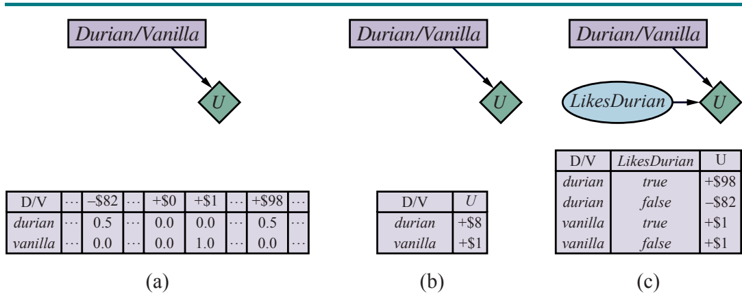
Figure 16.10 (a) A decision network for the ice cream choice with an uncertain utility function. (b) The network with the expected utility of each action. (c) Moving the uncertainty from the utility function into a new random variable.
