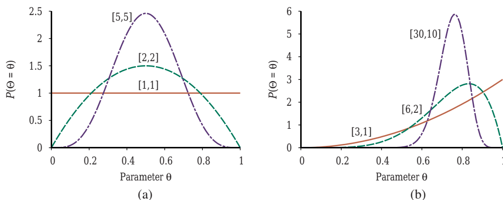
Figure 20.5 Examples of the Beta(a, b) distribution for different values of (a, b) .
