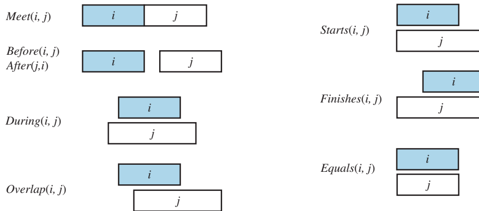
Figure 10.2 Predicates on time intervals.
