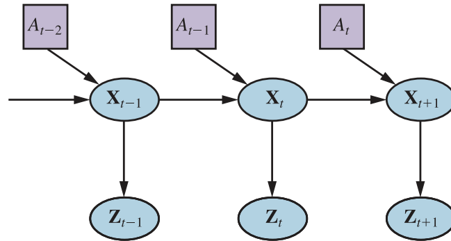
Figure 26.4 Robot perception can be viewed as temporal inference from sequences of actions and measurements, as illustrated by this dynamic decision network.
